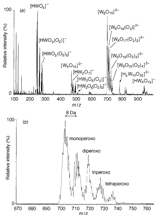
Fig. 6 (a) The ESI mass spectrum of a solution of peroxide + tungsten metal, 1 mmol dm -3 in W, pH ca. 2. The [W 6 O 19 ] 2- anion peak is observed in this spectrum and, in addition, the species generated from one to four peroxo substitutions, i.e. [W 6 O 18 (O 2 )] 2- , [W 6 O 17 (O 2 ) 2 ] 2- , [W 6 O 16 (O 2 ) 3 ] 2- and [W 6 O 15 (O 2 ) 4 ] 2- . (b) Expansion of the [W 6 O 19 ] 2- ion peak and its peroxo analogues which clearly shows the separation of m/z = 8 between adjacent peaks
